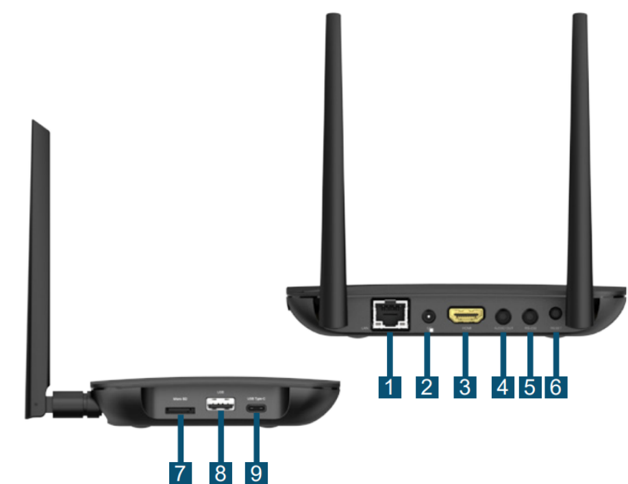
Hardware Ports
